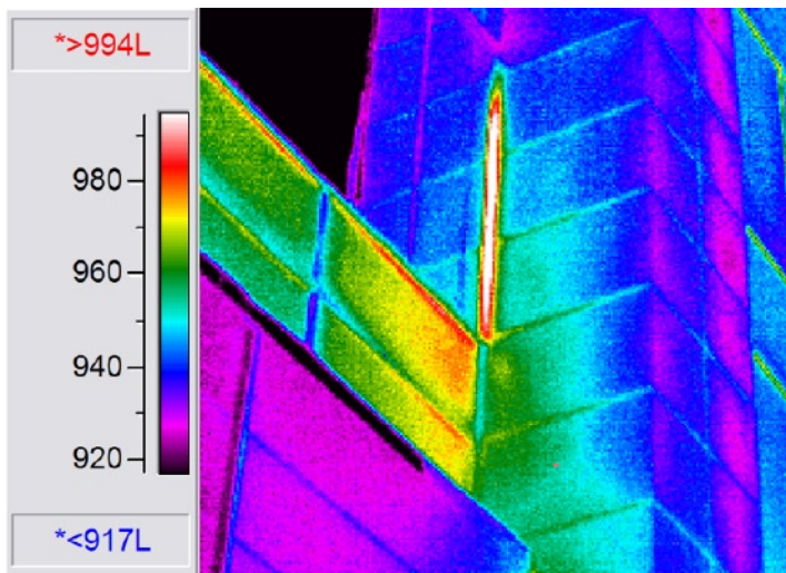
Thermogram #2 - “Stack Effect” is exacerbated by significant warm air exfiltration near the top of the building.
