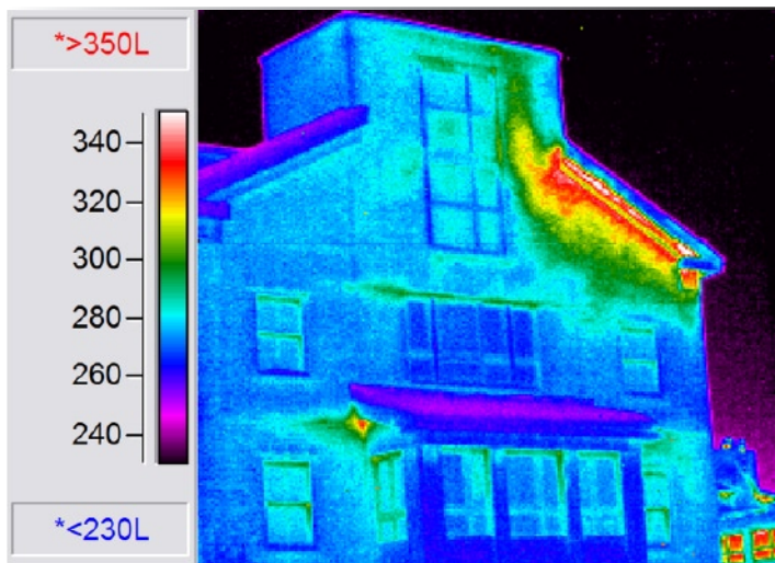
Thermogram #7 - Thermographic evaluations of new construction often reveal significant building envelope problems.
