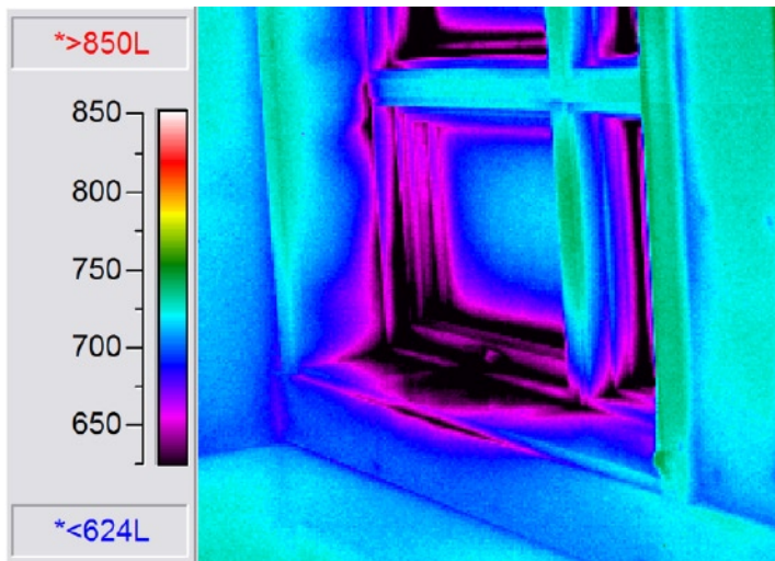
Thermogram #6 - Even newly installed windows can have serious performance issues.
