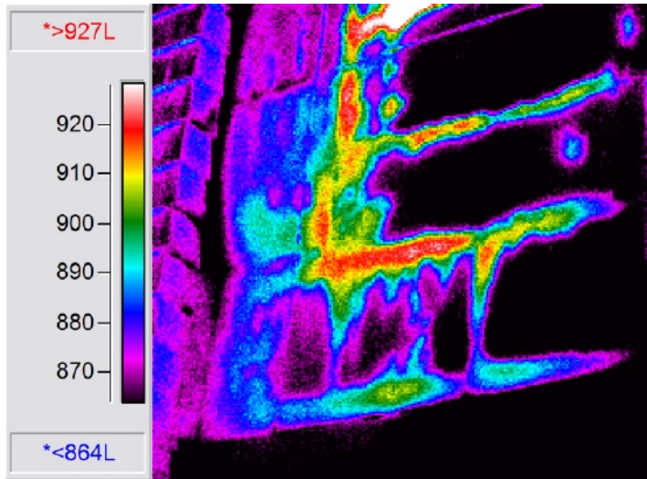
Thermogram #4 - Thermography is an ideal tool for isolating water-damaged areas in EIFS systems.
